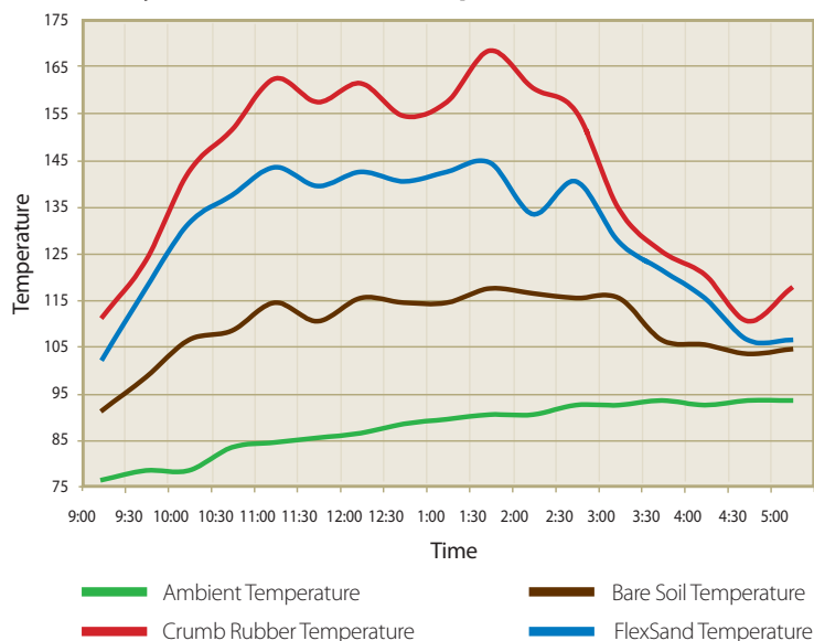
Synthetic Turf Surface Temperature with No Wind
